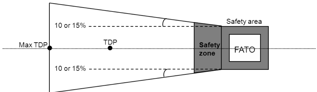
Figure 2: Obstacle accountability
