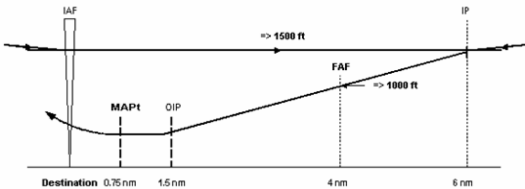
Figure 5: Missed approach area left & right
