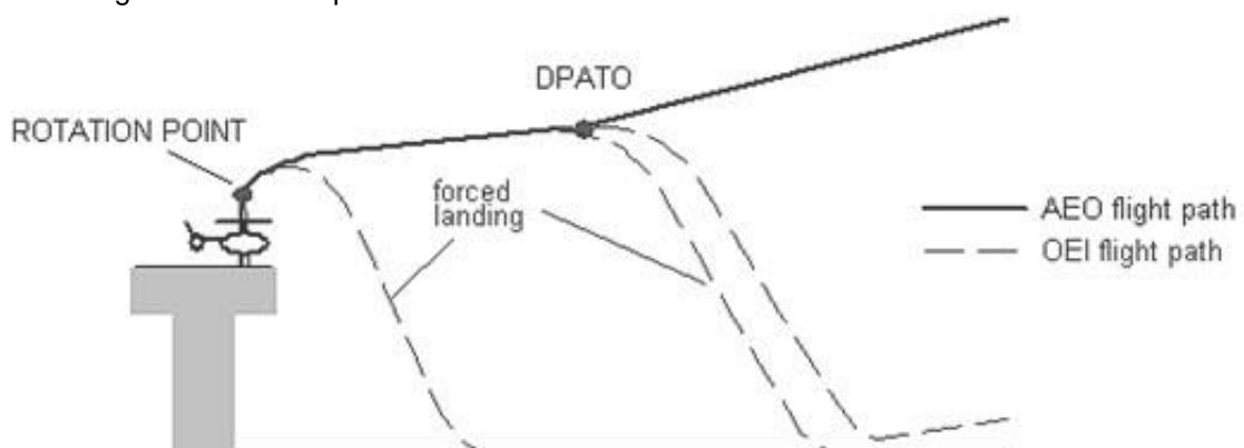
Figure 1: Take-off profile
