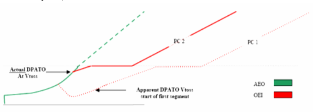
Figure 8: Using Cat A data; actual and apparent position of DPATO ( V_{\text{toss}} and start of first segment)
