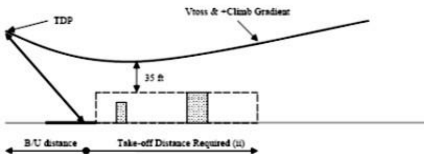
Figure 3: Helipad take-off
