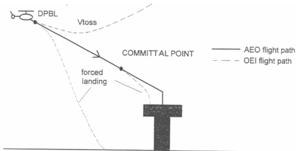
Figure 2: Standard landing profile
