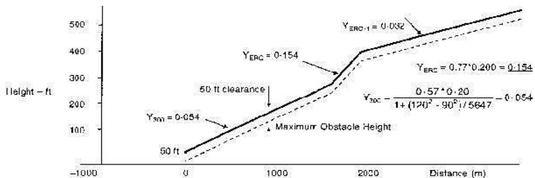
Figure 3: Assumed engine failure height less than 200 ft
