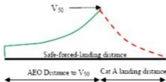
Figure 10: Category B (V50) safe–forced–landing distance
