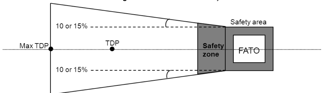
Figure 2: Obstacle accountability
