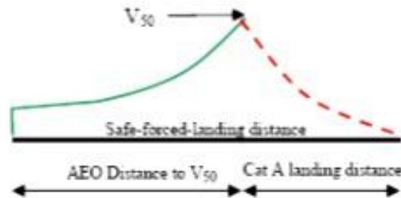
Figure 10: Category B (V50) safe-forced-landing distance
