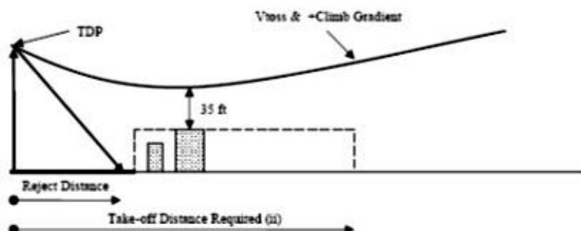
Figure 2: Short Field take- off
