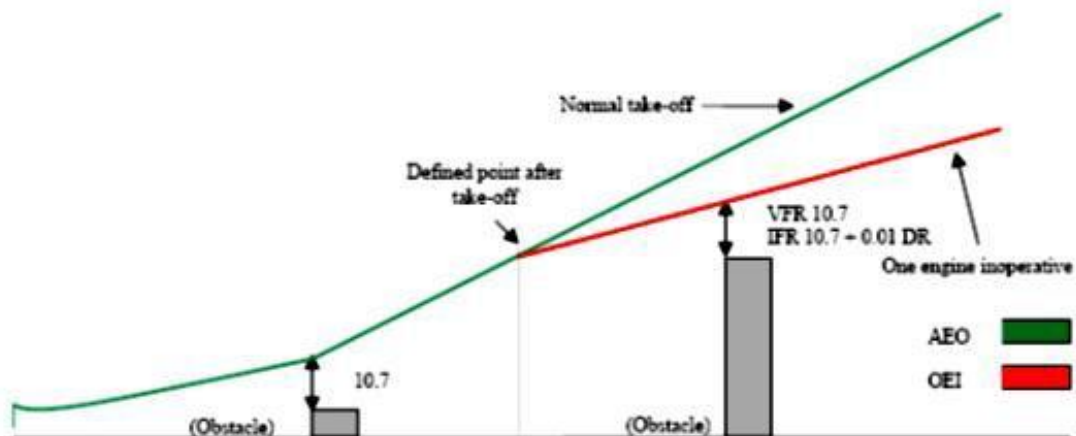
Figure 3: Performance Class 2 Obstacle Clearance
