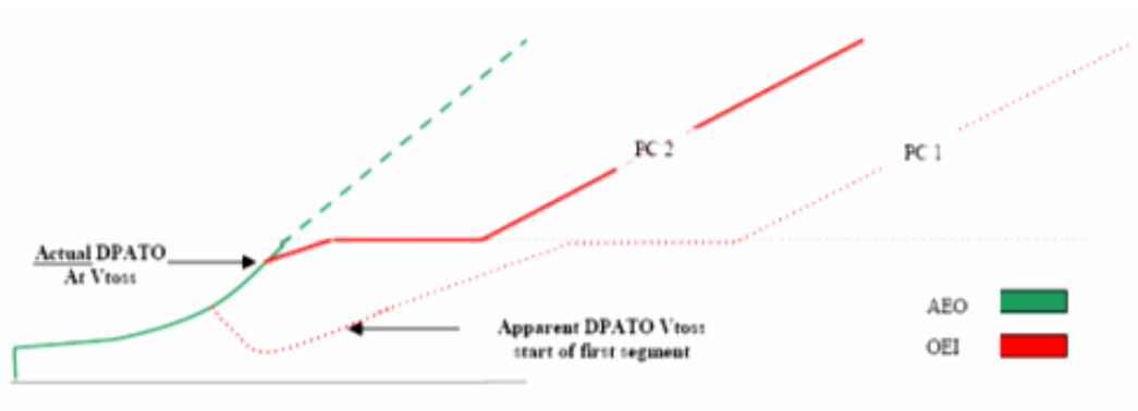
Figure 8: Using Cat A data; actual and apparent position of DPATO (V toss and start of first segment)
